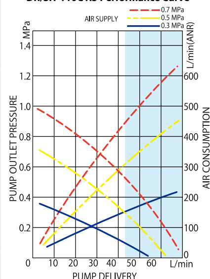
DR/SH-110C1.5 Performance Curve
