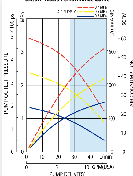
DR/SH-125B5 Performance Curve
