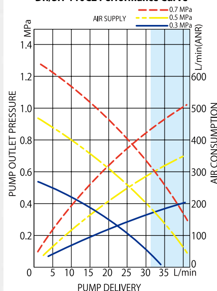
DR/SH-110C2 Performance Curve
