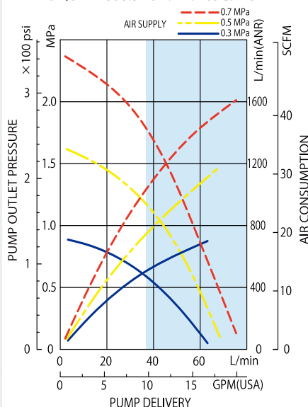
DR/SH-125B3.5 Performance Curve
